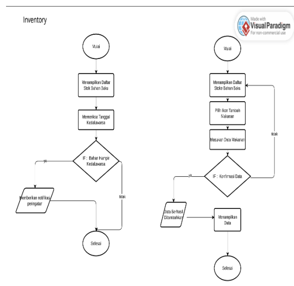
Figure 4. flowchart fitur inventory
