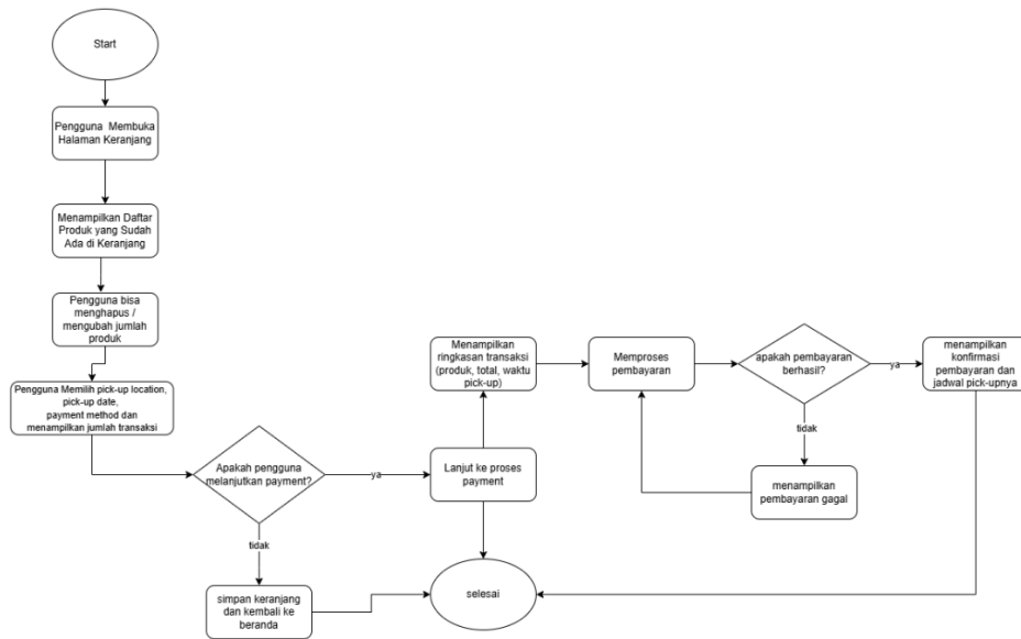
Figure 5. flowchart fitur transaksi
